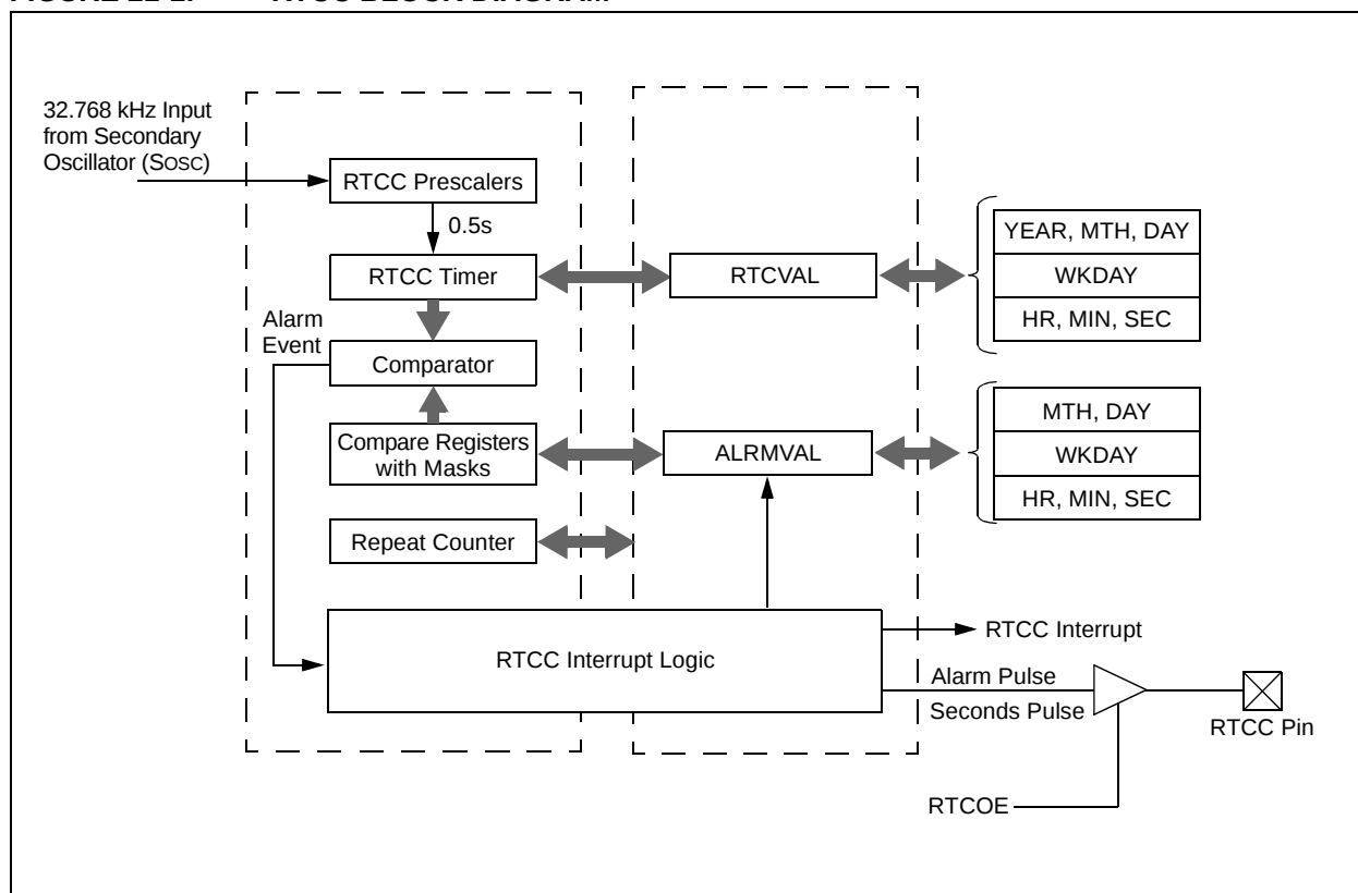
FIGURE 21-1: RTCC BLOCK DIAGRAM
