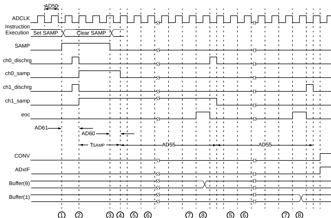
FIGURE 31-19: A/D CONVERSION (10-BIT MODE) TIMING CHARACTERISTICS (CHPS<1:0> = 01, SIMSAM = 0, ASAM = 0, SSRC<2:0> = 000)
